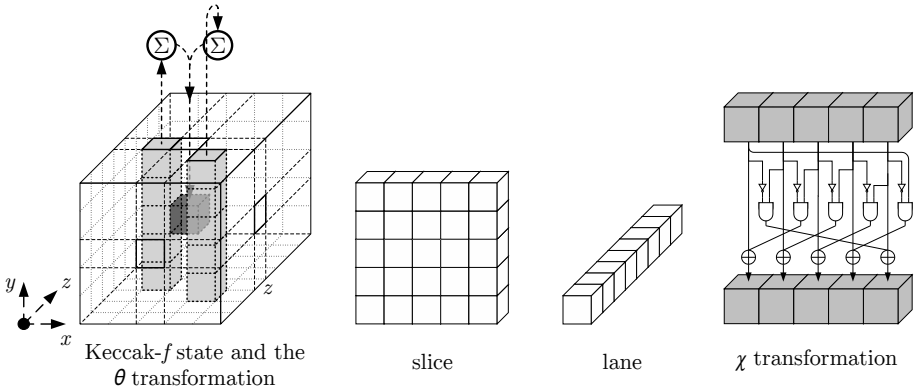
Fig. 1: Parts of the KECCAK- f state [5] including \theta transformation (left) and \chi transformation (right) 2
